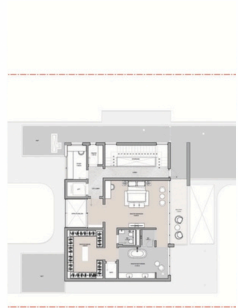
6-Bedroom villa type A- Second floor plan
