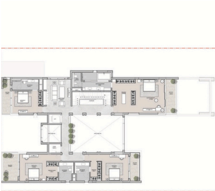
6-Bedroom villa type A- First floor plan
